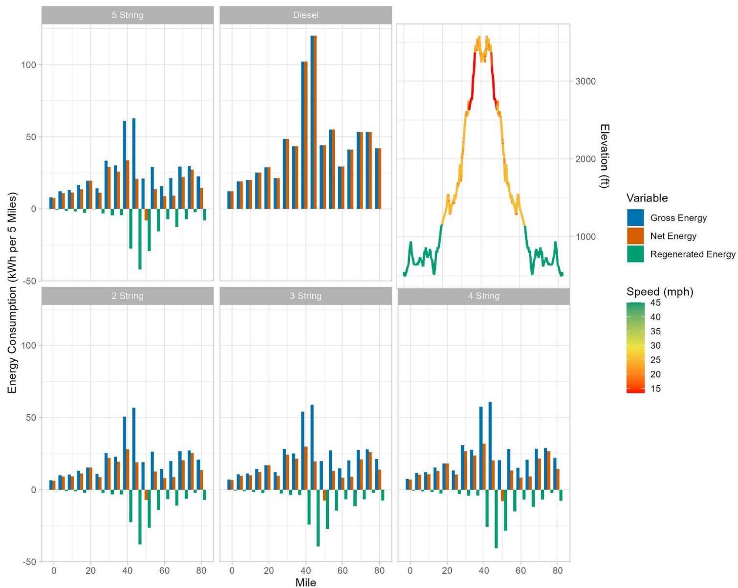
Figure D4: Round trip elevation, speed and energy cost (kWh) bar charts at 5mi intervals for the Scott Turner Road from the Vener mill for every vehicle configuration
